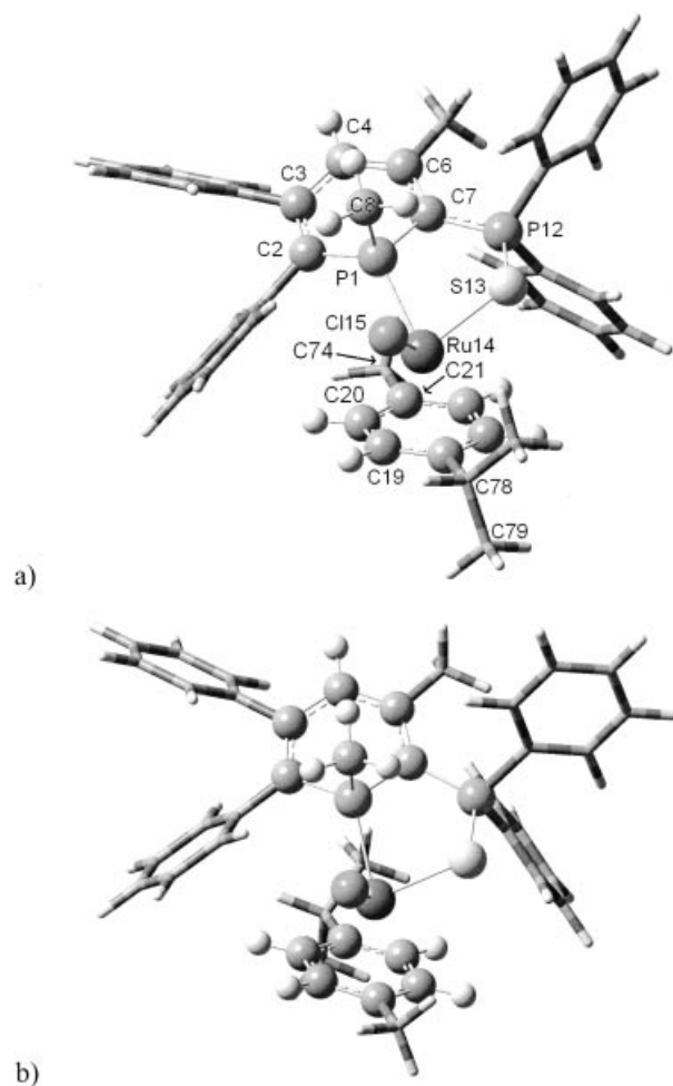
Figure 3. Optimized structures of model complexes Ia (a) and Ib (b) obtained at the ONIOM(B3LYP/UFF) level of theory; atoms included in the QM part are shown in ball-and-stick format and atoms included in the MM part are represented by tubes; the numbering is the same for Ia and Ib
