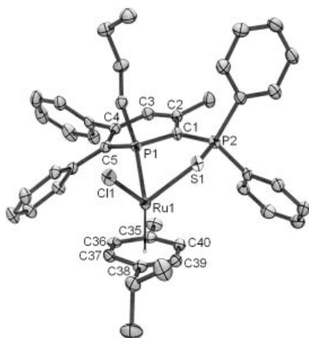
Figure 2. ORTEP view of a molecule of complex 5a ; ellipsoids are scaled to enclose 50% of the electron density; the numbering is arbitrary and different from that used in the assignment of the NMR spectra; selected distances [Å] and bond angles [°]: P1–C1 1.790(2) , C1–C2 1.422(3) , C2–C3 1.372(3) , C3–C4 1.435(2) , C4–C5 1.376(3) , C5–P1 1.805(2) , P1–Bu 1.852(2) , C1–P2 1.745(2) , P2–S1 2.0283(7) , Ru1–P1 2.3351(5) , Ru1–S1 2.4239(5) , Ru1–Cl1 2.4186(5) , Ru1–C35 2.237(2) , Ru1–C36 2.239(2) , Ru1–C37 2.196(2) , Ru1–C38 2.276(2) , Ru1–C39 2.257(2) , Ru1–C40 2.189(2) , Ru1–Ct 1.725 , C35–C36 1.442(3) , C36–C37 1.401(3) , C37–C38 1.420(3) , C38–C39 1.408(3) , C39–C40 1.430(3) , C40–C35 1.402(3) , P1–C1–C2 121.1(1) , C1–C2–C3 122.5(2) , C2–C3–C4 125.3(2) , C3–C4–C5 125.1(2) , C4–C5–P1 119.2(1) , C5–P1–C1 102.82(8) , P1–C1–P2 111.9(1) ; (mean plane C1–C2–C4–C5)–P1 12.55 , (mean plane C1–C2–C4–C5)–C3 1.75
