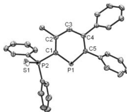
Figure 1. ORTEP view of a molecule of ligand 3 ; ellipsoids are scaled to enclose 50% of the electron density; the numbering is arbitrary and different from that used in the assignment of the NMR spectra; selected distances [Å] and bond angles [°]: P1–C1 1.739(2), C1–C2 1.406(2), C2–C3 1.395(2), C3–C4 1.392(2), C4–C5 1.404(2), C5–P1 1.736(2), C1–P2 1.824(2), P2–S1 1.954(1); P1–C1–C2 124.4(1), C1–C2–C3 120.8(2), C2–C3–C4 126.6(2), C3–C4–C5 121.7(2), C4–C5–P1 123.9(1), C5–P1–C1 102.60(7), P1–C1–P2 115.1(1); (mean plane C1–C2–C4–C5)–P1 0.45, (mean plane C1–C2–C4–C5)–C3 0.8
