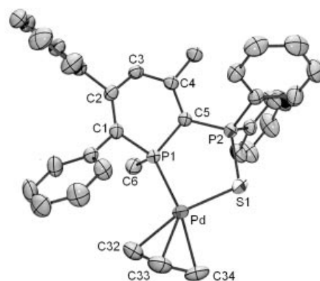
Figure 4. ORTEP view of one molecule of complex 7a ; ellipsoids are scaled to enclose 50% of the electron density; the numbering is arbitrary and different from that used in the assignment of the NMR spectra; selected distances [Å] and bond angles [°]: P1–C1 1.802(2), C1–C2 1.360(3), C2–C3 1.444(3), C3–C4 1.378(3), C4–C5 1.422(3), C5–P1 1.756(2), P1–C6 1.828(2), C5–P2 1.733(2), P2–S1 2.0288(8), Pd1–P1 2.2778(6), Pd–S1 2.3371(6), Pd–C32 2.138(3), Pd–C33 2.137(3), Pd–C34 2.199(3), C32–C33 1.359(4), C33–C34 1.383(5); P1–C1–C2 117.2(2), C1–C2–C3 123.4(2), C2–C3–C4 124.5(2), C3–C4–C5 121.0(2), C4–C5–P1 117.5(2), C5–P1–C1 101.7(1), P1–C5–P2 117.8(1), C32–C33–C34 123.8(3); (mean plane C1–C2–C4–C5)–P1 21.7; (mean plane C1–C2–C4–C5)–C3 7.3
